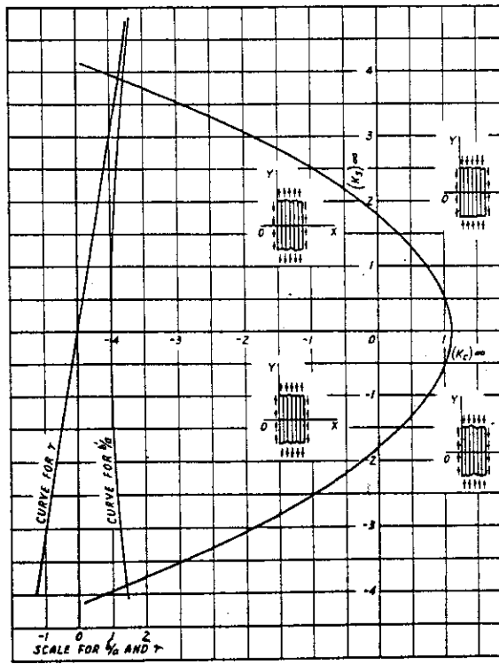
(h) 9-PLY (1:2:2:2:2:2:2:1) \beta = 0^\circ
