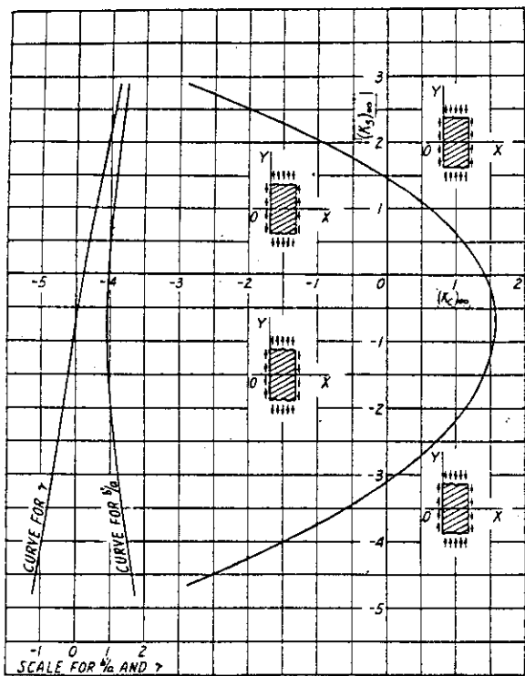
(e) 9-PLY (1:1:1:1:1:1:1) \beta = 60^\circ
