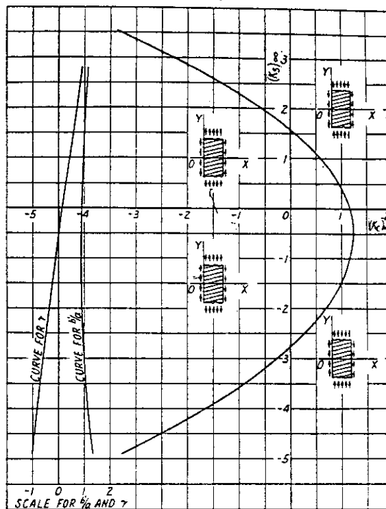
(f) 9-PLY (1:1:1:1:1:1:1) \beta = 75^\circ
