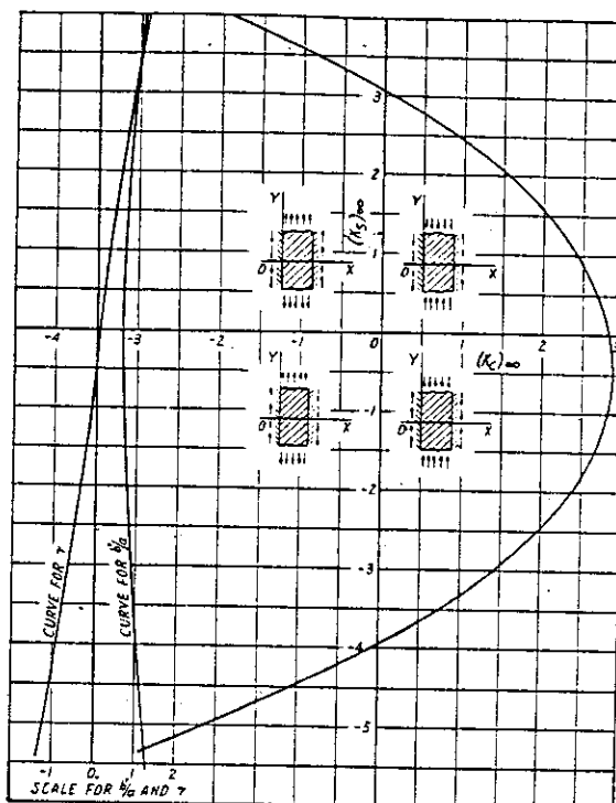
(e) 6-PLY (1:2:2:2:1) \beta = 45^\circ
