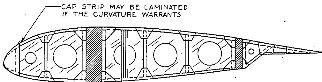
LIGHTENED PLYWOOD WEB TYPE
