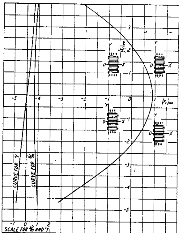
(p) 3-PLY (1:2:1) B=90^\circ
