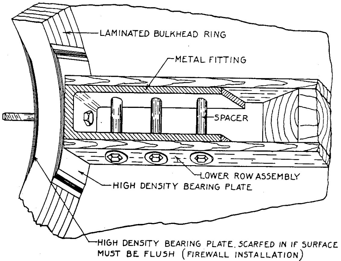
Figure 4-62. Typical fuselage joint or engine mount attachment.
