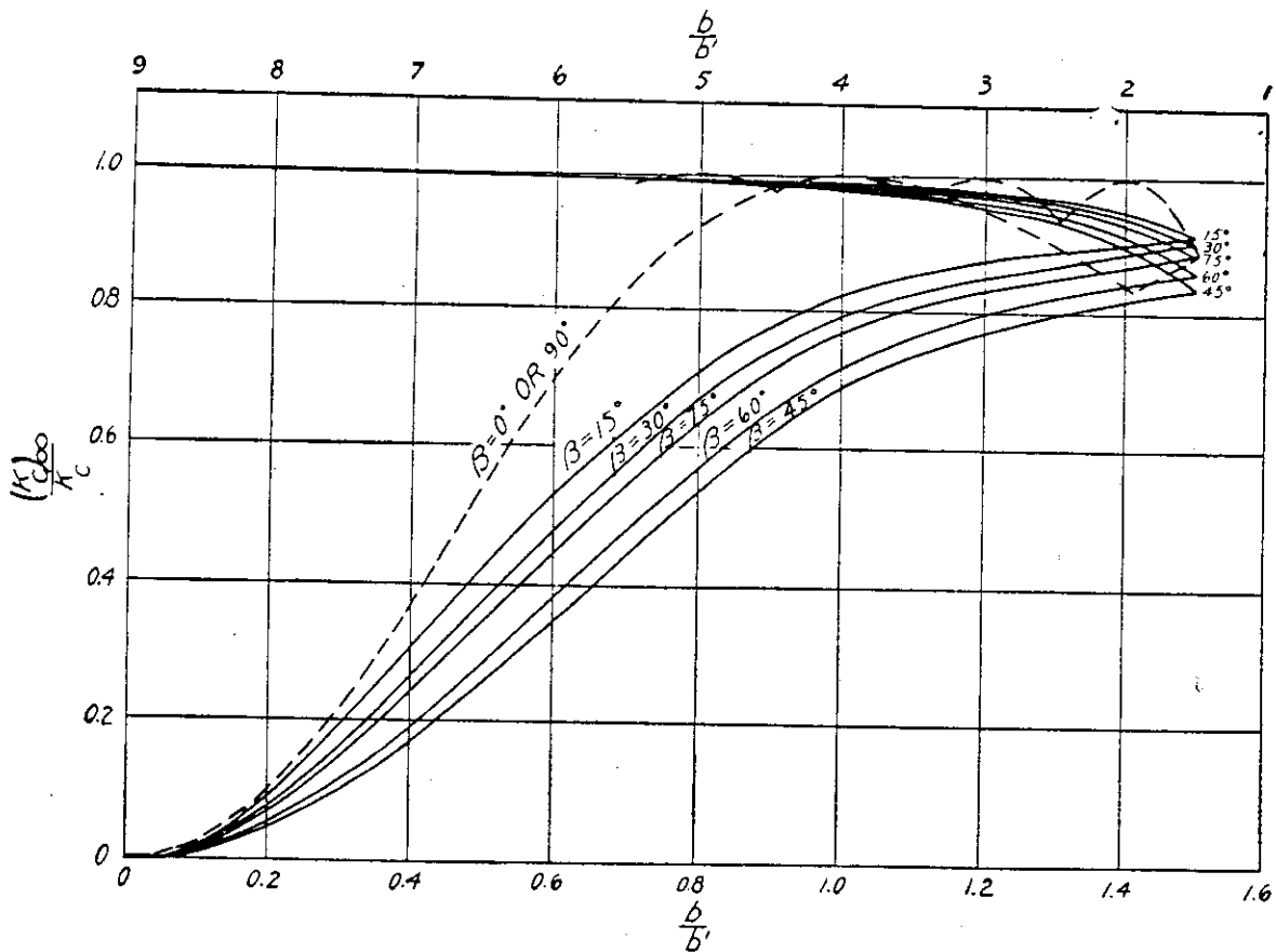
Figure 2-37. Corrections for panel size: Top, when \beta = 0^\circ, 45^\circ, or 90^\circ and panel is subjected to shear stress; bottom, when the panel is subjected to compression with the edges simply supported and \beta = 0^\circ or 90^\circ is a computed curve (ref. 2-50).
