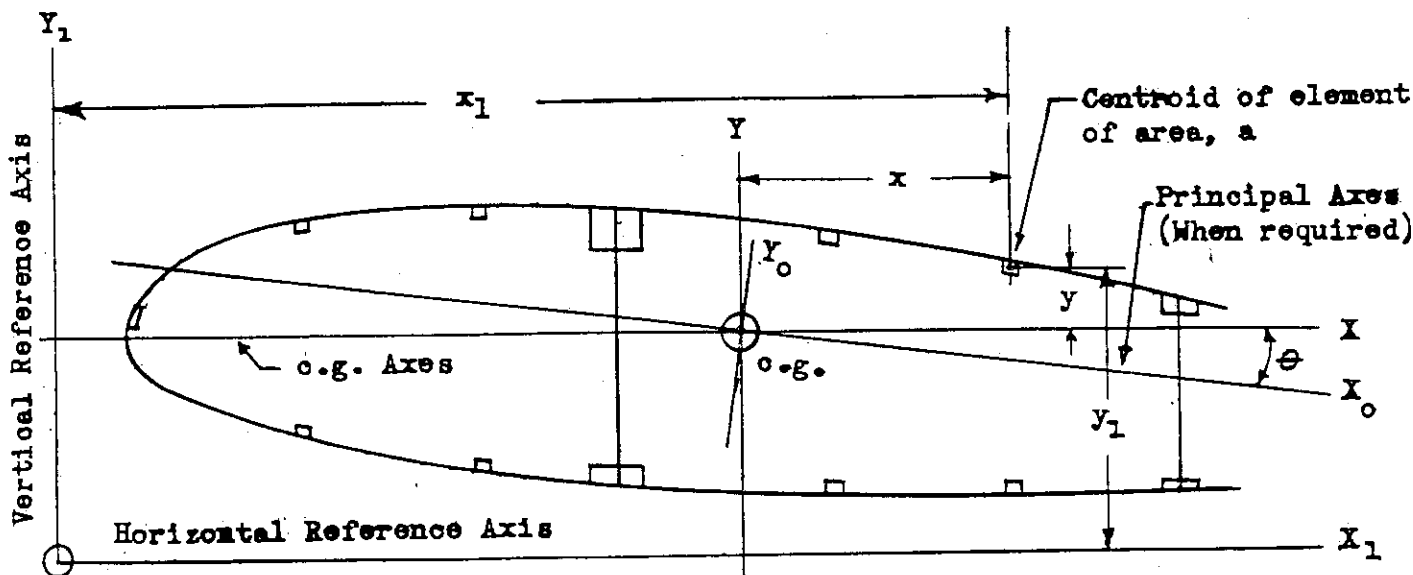
Figure 3-12. Diagram for computation of section properties.
