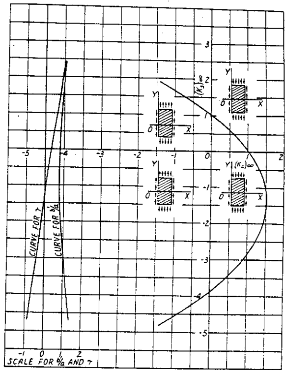
(m) 3-PLY (1:2:1) B=60^\circ
