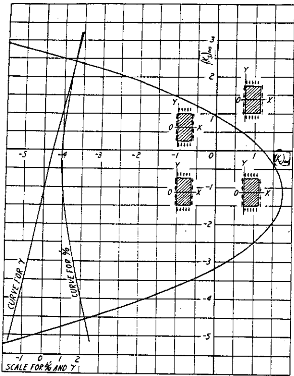
(k) 3-PLY (1:2:1) B=45^\circ
