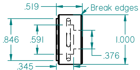
Outside Axle Spacer
